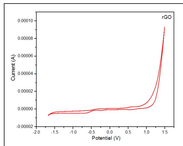
Fig. 12: Cyclic voltammetry analysis of rGO
