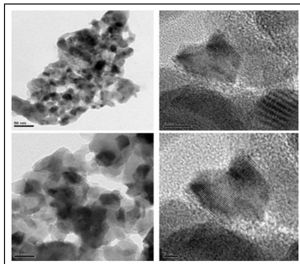
Fig. 2: TEM Images of Green Synthesized ZnO Nanoparticles
