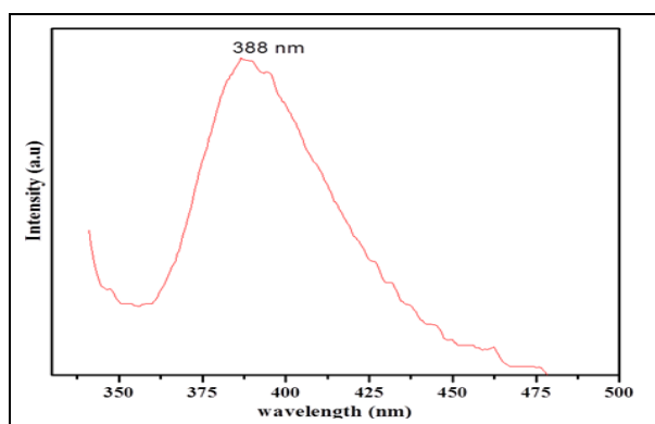
Fig. 5: Room Temperature PL Spectrum of Green Synthesized ZnO Nanoparticles
