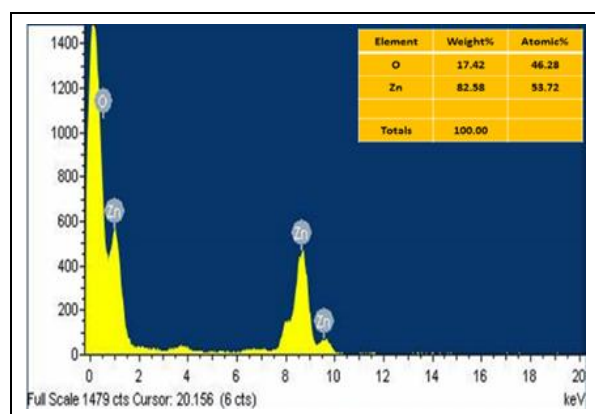
Fig. 3: EDAX Analysis of Green Synthesized ZnO Nanoparticles
