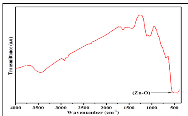
Fig. 4: FTIR Analysis of Green Synthesized ZnO Nanoparticles
