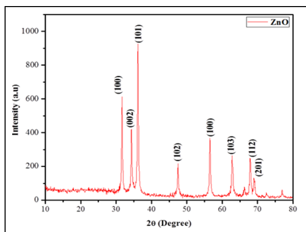
Fig. 1: XRD Pattern of Green Synthesized ZnO Nanoparticles
