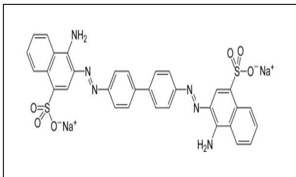
Structure of Congo red dye
