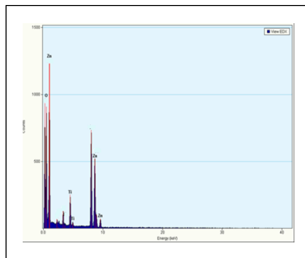
Fig. 5: EDAX of Flower like ZnO/TiO 2 nanocomposite
