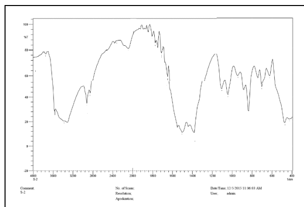
Fig. 2: FT-IR Spectrum of Flower like ZnO/TiO 2 nanocomposite
