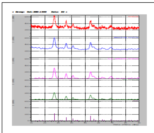
Fig. 3: XRD of Flower like ZnO/TiO 2 nanocomposite
