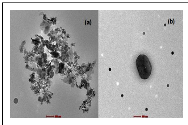
Fig. 6: TEM analysis of Flower like ZnO/TiO 2 nanocomposite
