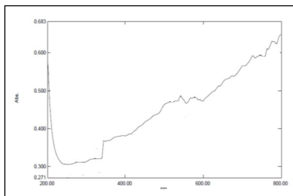
Fig. 1: UV spectrum of ZnO/TiO 2 nano composite
