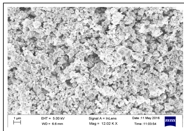
Fig. 5: SEM image of CuO Composite nanoparticles with polymer isopropanol
