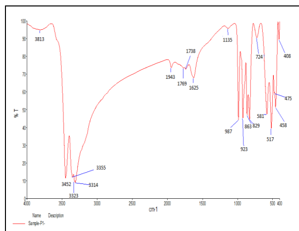
Fig. 3: FTIR spectra of copper oxide nanocomposite synthesized by refluxing method
