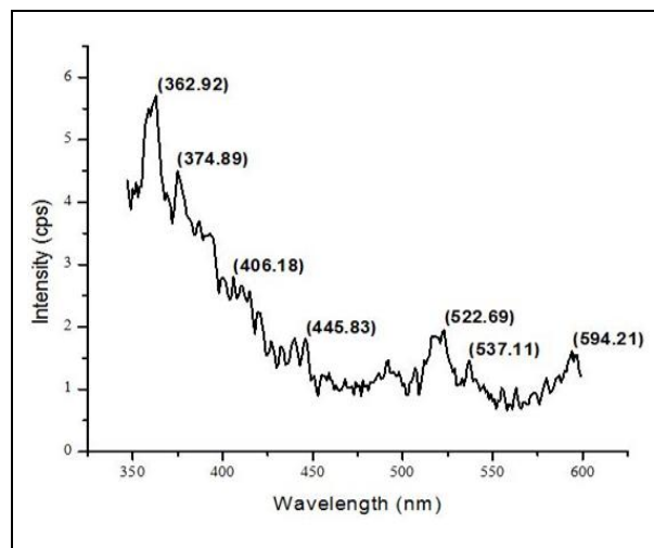
Fig. 2: Photoluminescence spectra of copper oxide nanocomposite synthesized by refluxing method
