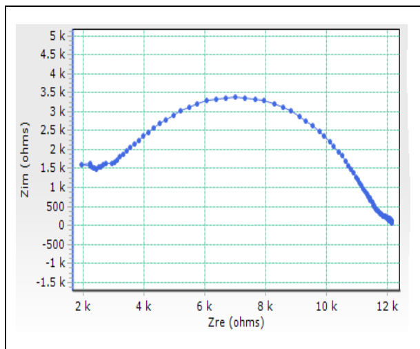
Fig. 4: Nyquist plot of copper oxide nanocomposite synthesized by refluxing method.
