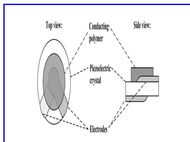
Fig. 10: Configuration of quartz crystal microbalance sensor device
