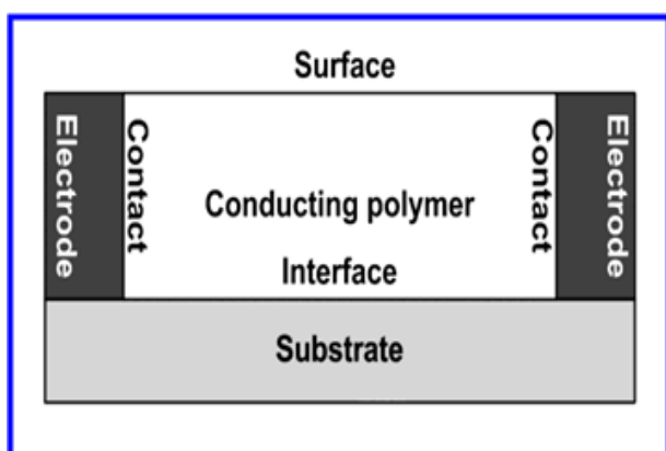
Fig. 9: Configuration of chemiresistor
