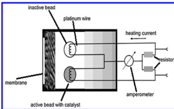
Fig. 1: Pellistor-type gas sensor (Hubert et al. 2011)
