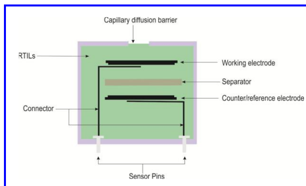
Fig. 3: Proposed membrane-free gas detector
