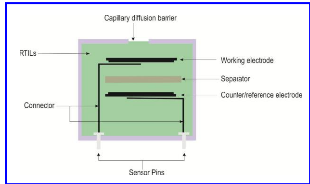
Fig. 3: Proposed membrane-free gas detector
