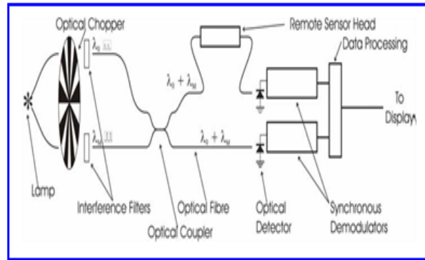
Fig. 5: Schematic of a differential fibre-optic detection system (Redrawn from diagram in Hordvik et al. 1983)
