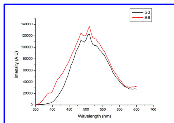
Fig. 4: Comparison of PL Spectra of GTE Film
