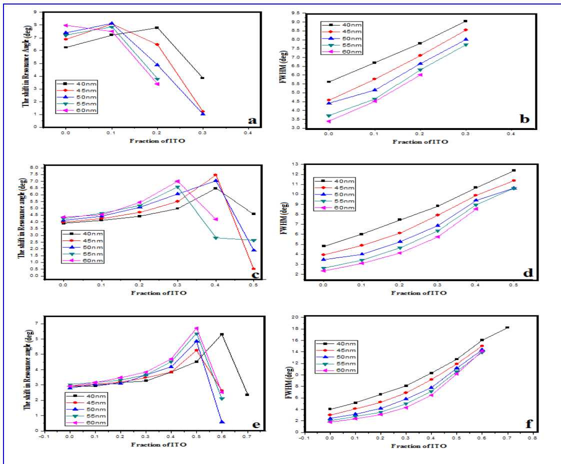
Fig. 2: Variations of the shift in resonance angle and FWHM of prism based SPR sensor for ITO hosted on the dielectric metal gold (a)and(b) for the prism of n_p=1.456 (c)and(d) for the prism of n_p =1.51391 (e)and(f) for the prism of n_p =1.597
