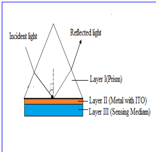
Fig. 1: Schematic diagram of prism based SPR sensor
