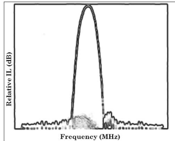
Fig. 3 : Frequency response of SAW Filter
